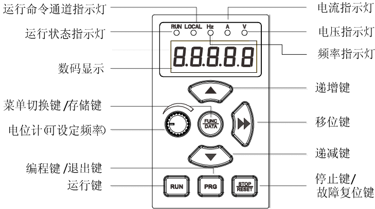
C3000-2S0007G~C3000-2T0022G LED 操作面板示意图
